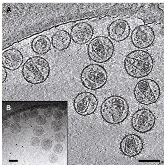
The Mechanism of HIV-1 Core Assembly: Insights from Three-Dimensional Reconstructions of Authentic Virions Structure VOLUME 14, ISSUE 1, P15-20, JANUARY 01, 2006
